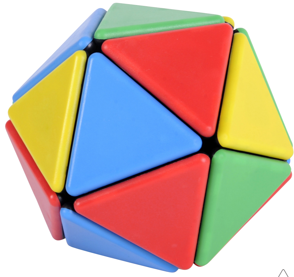
Icosahedron
